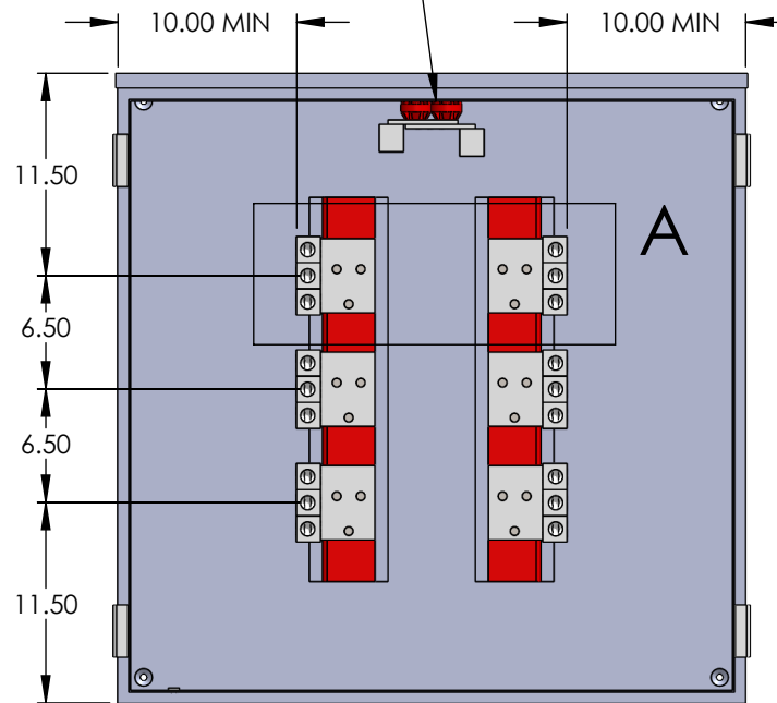
FRONT VIEW OPENED
